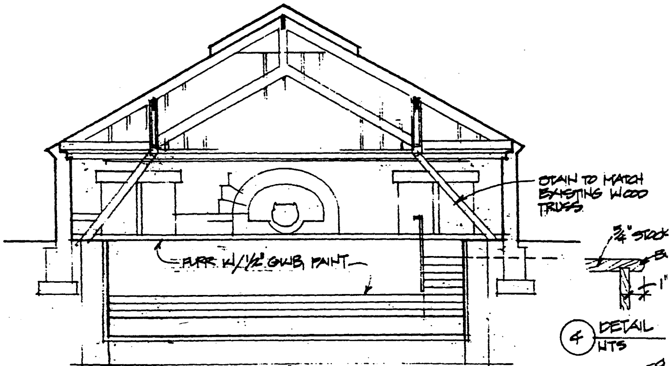
2 SECTION 1/8'
